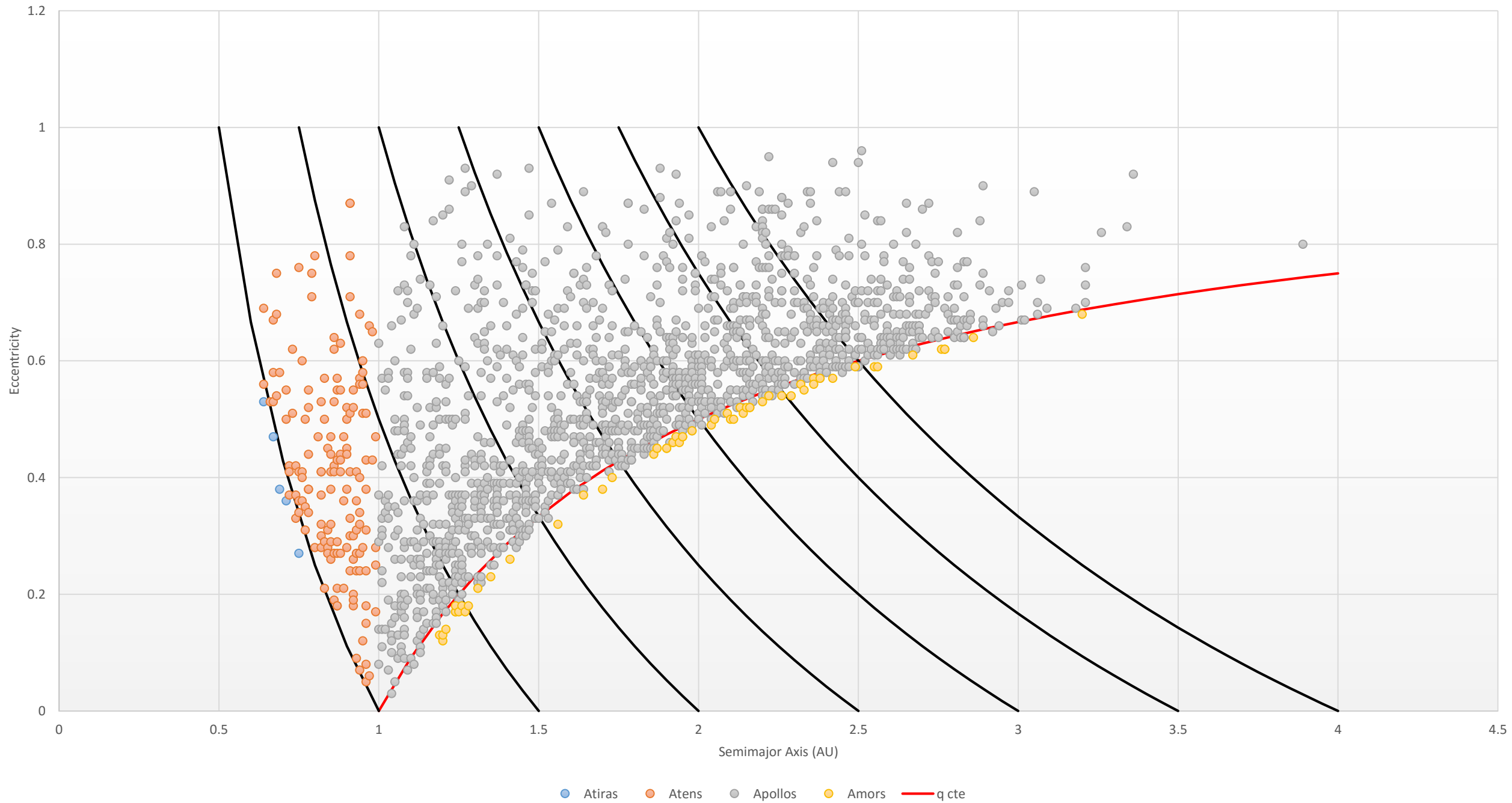
Potentially Hazardous Asteroids (PHAs)
